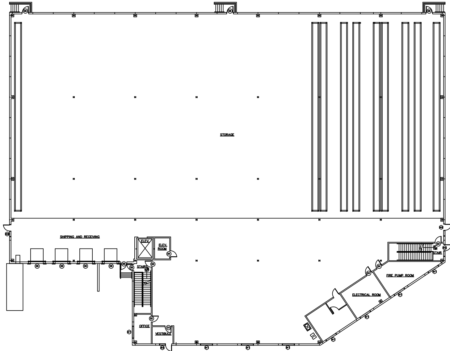
AVAILABLE SPACE GROUND FLOOR PLAN
